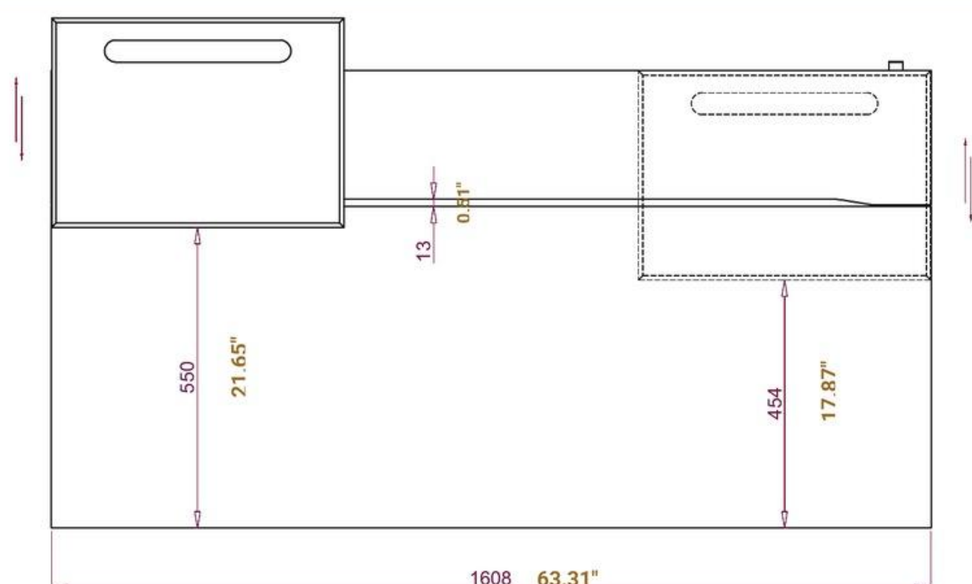
TOP VIEW – FOOTPRINT
