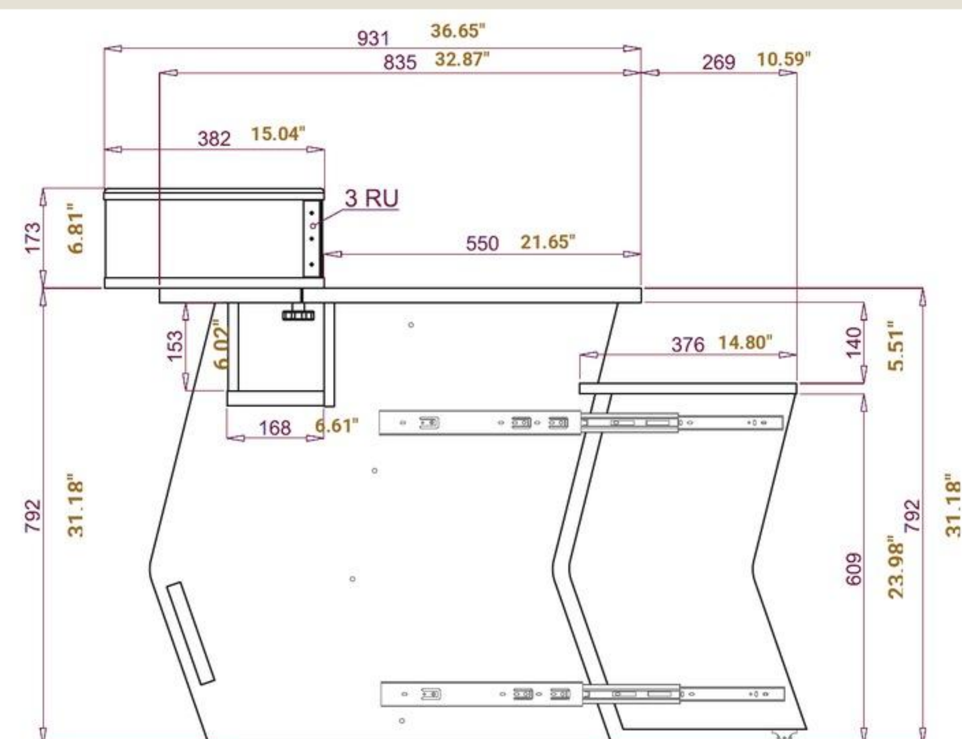
SIDE VIEW WITH OPEN KEYBOARD
