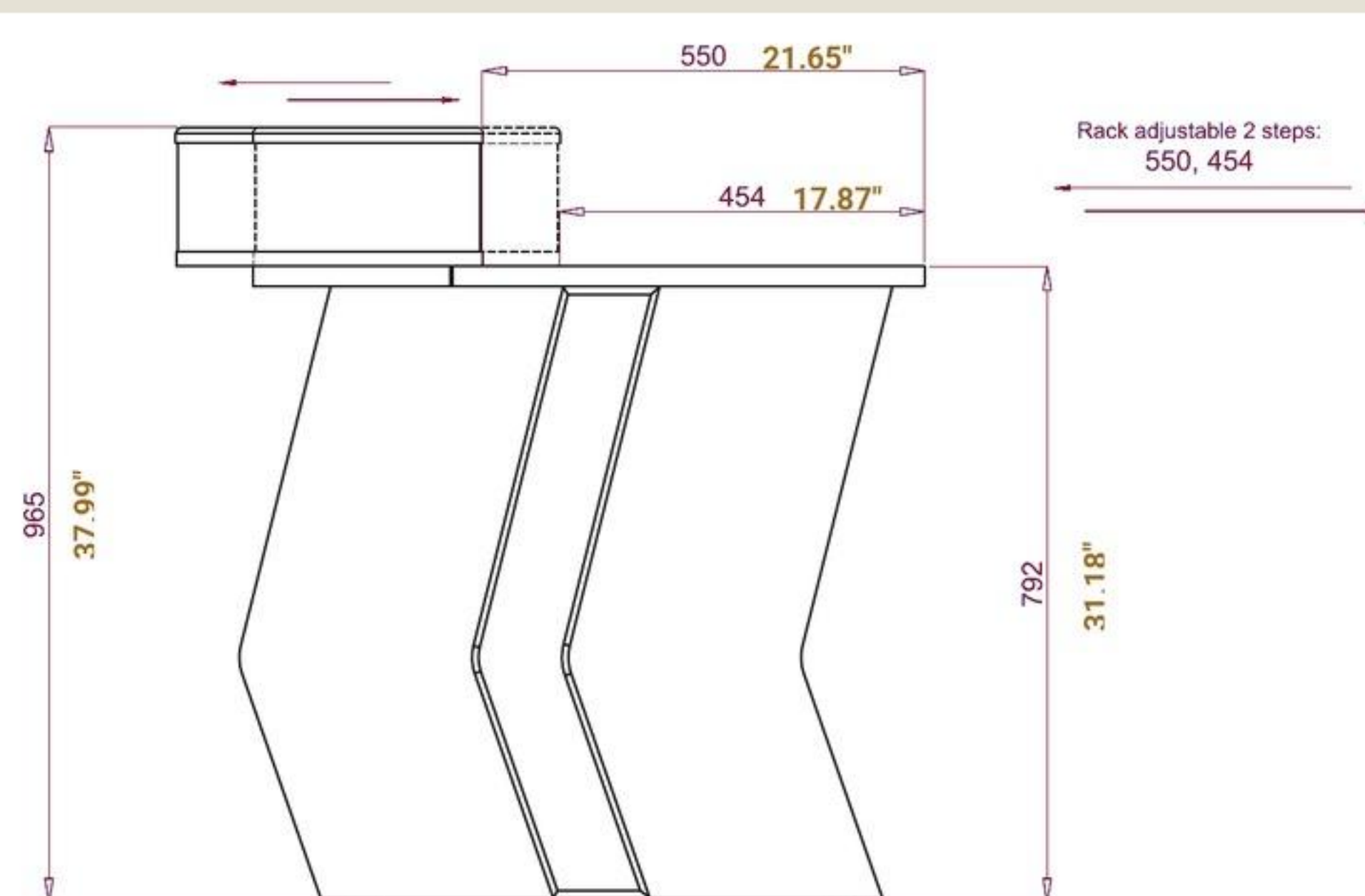
SIDE VIEW WITH CLOSED KEYBOARD, 2 POSSIBLE POSITIONS OF RACK
