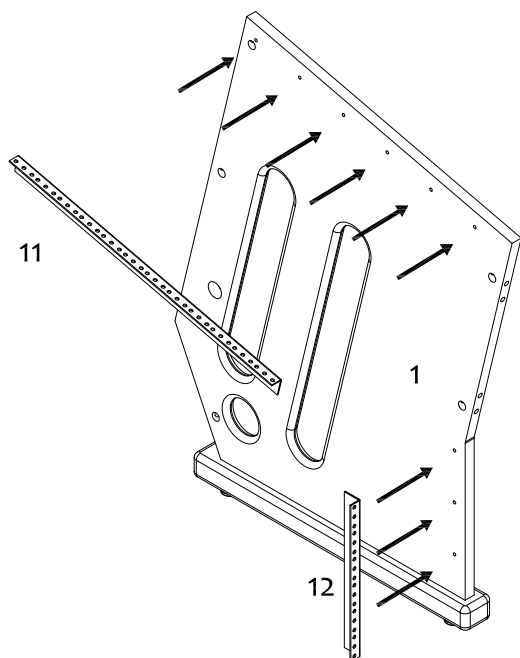
STEP 9: fix rail N° 11+12 with rail screws R
