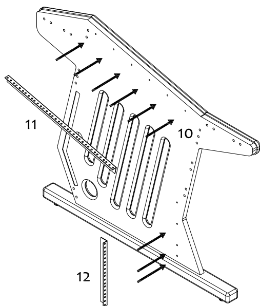
STEP 9: fix rail N° 11+12 with rail screws R
