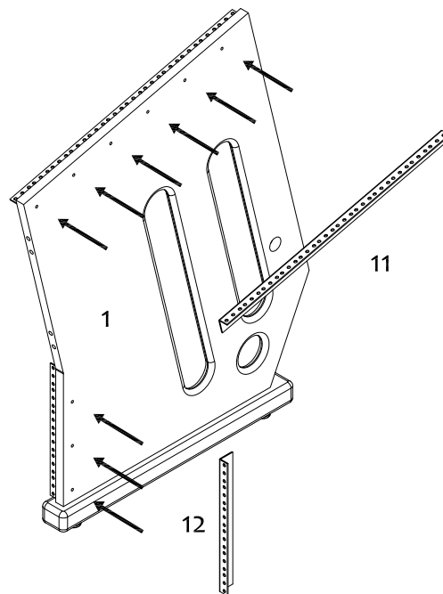
STEP 10: fix rail N° 11+12 with rail screws R
