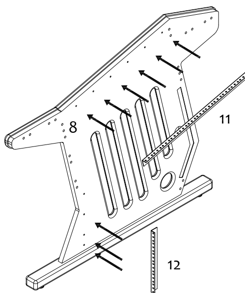
STEP 10: fix rail N° 11+12 with rail screws R
