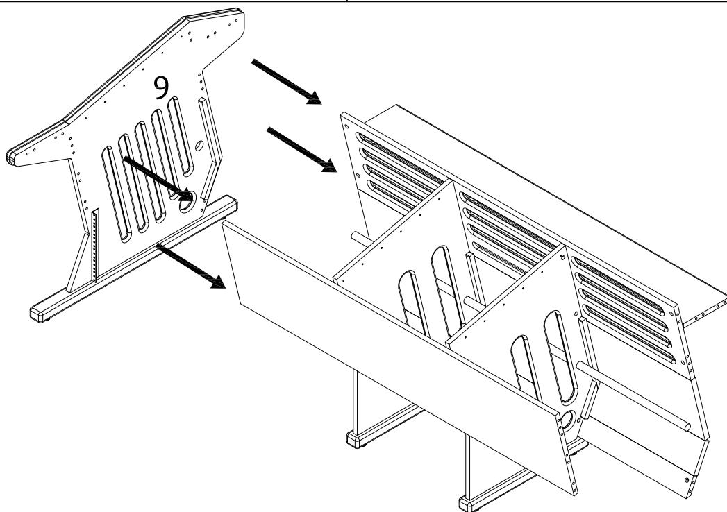
STEP 19
