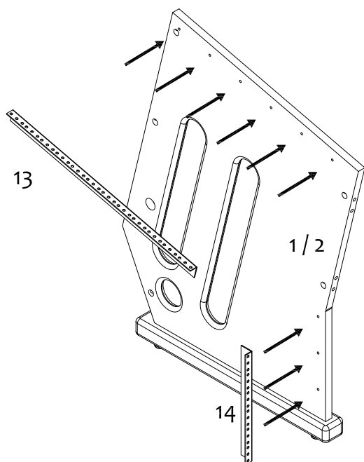
STEP 11: fix rail N° 11+12 with rail screws R. Repeat step for pieces N°2
