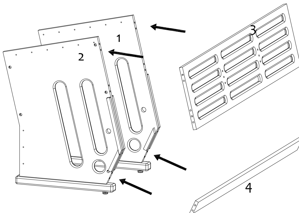
STEP 14: fix rail N° 11+12 with rail screws R
