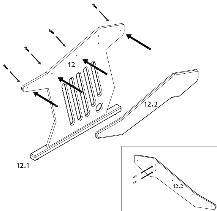
STEP 10: Insert the wood dowels in piece 12.2. Then fix piece N° 12.2 to 12 with screws B
