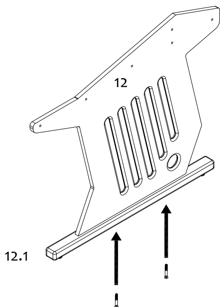
STEP 9: fix piece N° 12.1 with screws A
