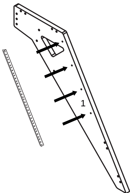
Step 1 Fix rack bar with screws Type R
